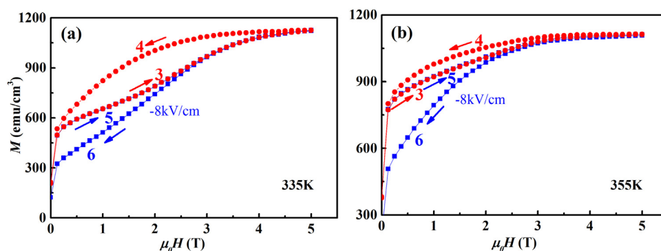
Fig. 8. Realization of an inverse hysteresis loss with electric field applied during the demagnetization process at 335 K (a) and 355 K (b). Path 3–4 denotes the M - H curve in the absence of electric field in the second cycle (the virgin effect has been eliminated, and path 1–2 does not show for clarify), while Path 5–6 denotes the subsequent cycle, where -8 \text{ kV cm}^{-1} is applied in the entire demagnetization process. One can notice the inverse hysteresis cycled by Path 5–6.
