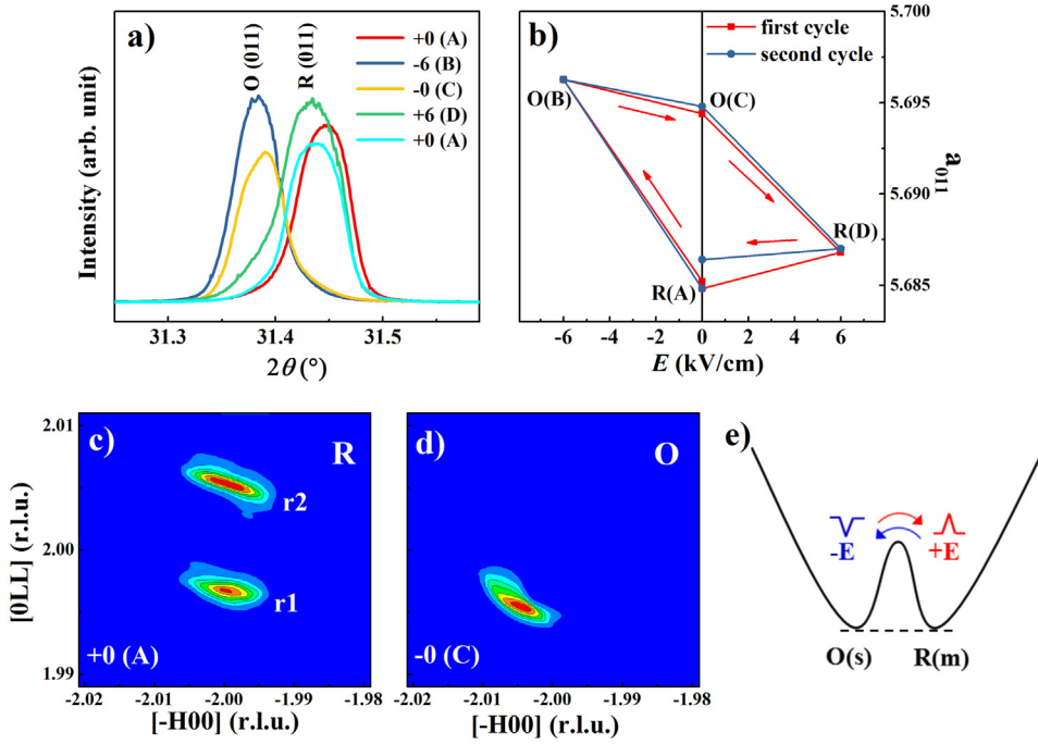
Fig. 5. (a) XRD patterns measured at room temperature, where the electric field E was in situ applied in the sequence of + 0, - 6, - 0, + 6, + 0 \text{kV cm}^{-1} . (b) The deduced lattice parameter a_{011} along the out-plane [011] direction versus E . Reciprocal space maps (RSMs) around the (-222) reflection of PMN-PT substrate for states of (c) + 0 and (d) - 0 \text{kV cm}^{-1} , where r1, r2 denote the domains of R phase. (e) Hypothetical Gibbs free energy profiles of multidomain R phase (R(m)) and single-domain O phase (O(s)). R, O denote rhombohedral and orthorhombic phase, respectively, while A, B, C, D in the brackets correspond to the ones in Fig. 3b.
