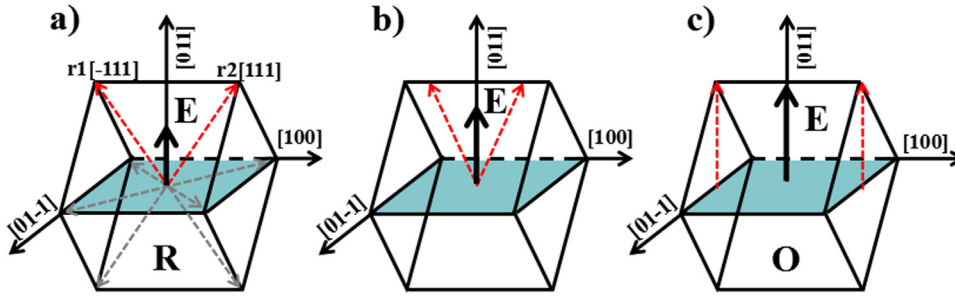
Fig. 4. The evolution of domain structure during the R-O phase transition for the PMN-PT single crystal with electric field E poled along [011] direction. (a) The arrows along the body diagonals denote the eight possible spontaneous polarization directions of R phase. The red arrows represent the polarization directions for (a) R phase, (b) intermediate phase, and (c) O phase.
