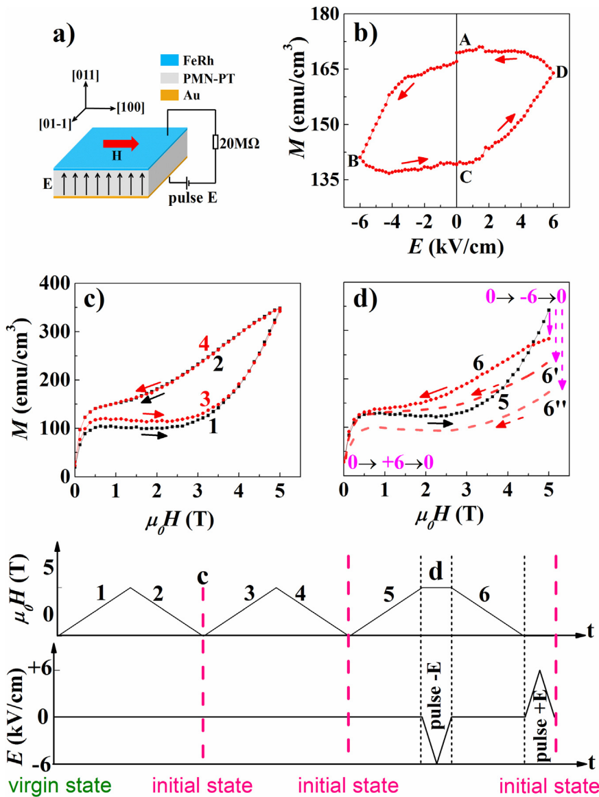
Fig. 3. (a) Sketch of the FeRh/PMN-PT heterostructure, where H and E denote the applied magnetic field and pulse electric field, respectively. (b) The loop-like M - E curve measured at 5 T and 310 K. (c) M - H curves in the virgin (path 1–2) and second (path 3–4) cycles in the absence of electric field, after that (d) path 5 from 0 to 5 T was continued and a pulse electric field 0 \rightarrow -6 \rightarrow 0 kV cm ^{-1} was applied to switch and memory the strain state at 5 T, then path 6 from 5 T to 0 was performed and followed by a pulse electric field 0 \rightarrow +6 \rightarrow 0 kV cm ^{-1} . Supposing the produced strain during 0 \rightarrow -6 \rightarrow 0 kV cm ^{-1} could be larger, path 6 would be along path 6' or path 6'' instead, and then the enveloped area by path 5–6' or 5–6'' would approach zero or turn out to be inverse. Lower panel, an exploded diagram corresponds to the above processes.
