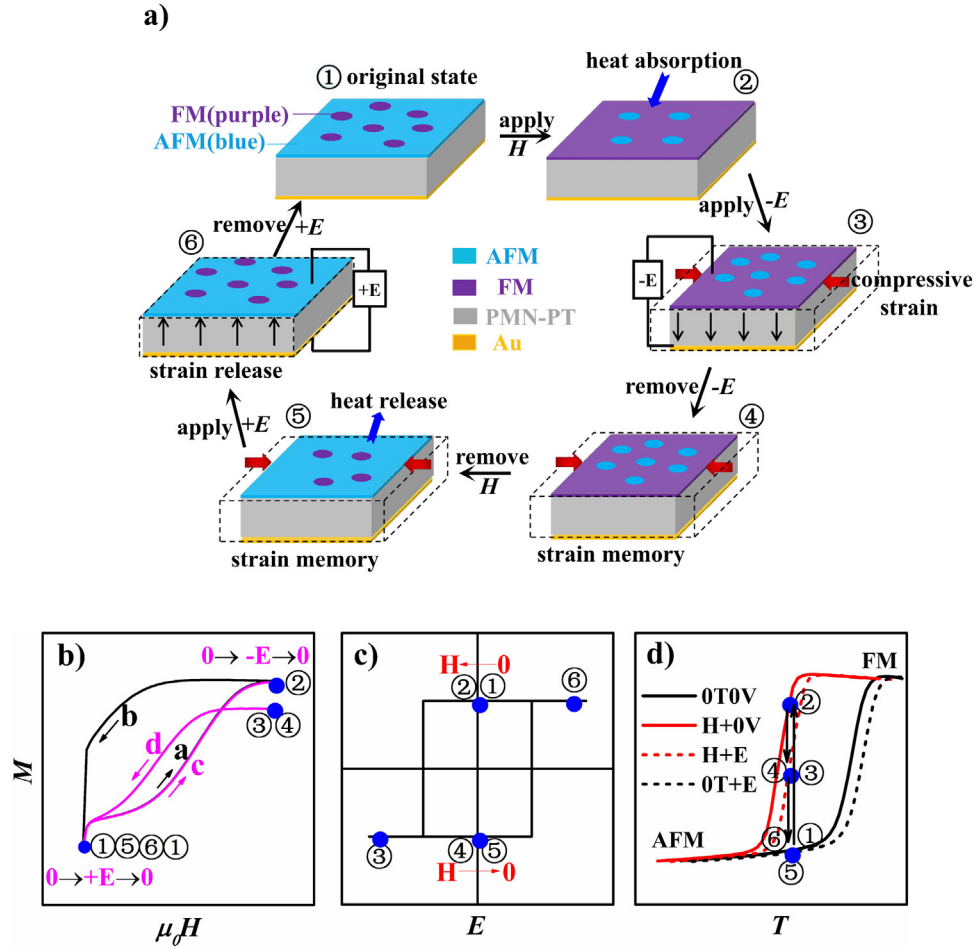
Fig. 1. Schematic of (a) refrigeration cycle, (b) M - H curves (after virgin cycle) with pulse \pm E applied only at points of 0 T and H , and the corresponding (c) M - E curves and (d) M - T curves at magnetic fields of 0 T and H .
