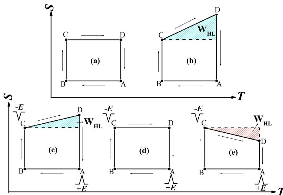
Fig. 7. S - T diagram of FeRh for an ideal magnetic Carnot cycle between T_h (A,D) and T_c (B,C) composed of two isothermal and two adiabatic processes: (a) Reversible Carnot cycle without considering hysteresis loss; (b) Carnot cycle considering full W_{HL} without pulse \pm E ; (c) Carnot cycle considering partially reduced W_{HL} with pulse -E , +E successively applied at points C, A; (d) Carnot cycle considering fully reduced W_{HL} = 0 with pulse \pm E ; (e) Carnot cycle considering inverse hysteresis loss, W_{HL} < 0 , with pulse \pm E . In the adiabatic processes, entropy does not remain constant because W_{HL} acts as an unavoidable entropy source [42]. For simplicity, the impact is only denoted in the C-D branch.
