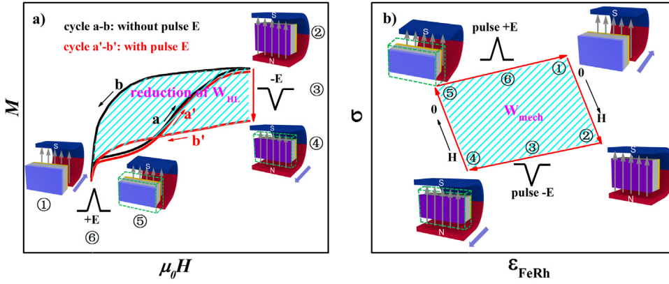
Fig. 6. Schematic of (a) the magnetic loops with (path a'-b') and without (path a-b) the applications of pulse \pm E , and (b) mechanical work (the shadow area), W_{mech} , during the refrigeration cycle, where the thin film stress \sigma versus in-plane strain \epsilon_{FeRh} is schematically shown. The cycled numbers correspond to the ones shown in Fig. 1.
