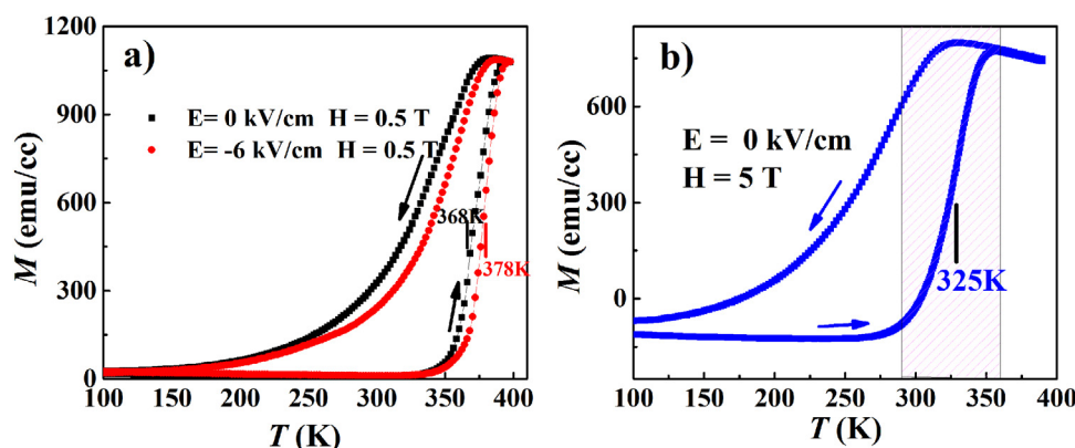
Fig. 2. (a) The M - T curves with and without application of -6 kV cm ^{-1} measured at 0.5 T. (b) The M - T curve at a high magnetic field of 5 T, where the shadow area signifies the phase transition region on heating.
