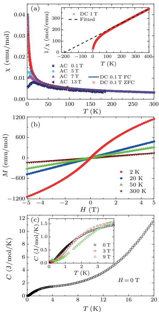
Fig. 2. (a) Temperature dependence of magnetic susceptibility under different magnetic fields measured by both DC and AC methods. In AC measurements, the oscillation field amplitude is 17 Oe and the oscillation frequency is 633 Hz. The inset shows the temperature dependence of the inverse susceptibility 1/\chi at 1 T. (b) Magnetic field dependence of magnetization at different temperatures. (c) Temperature dependence of the specific heat at zero field down to 50 mK. The inset shows the magnetic field effect on the specific heat at low temperatures.
