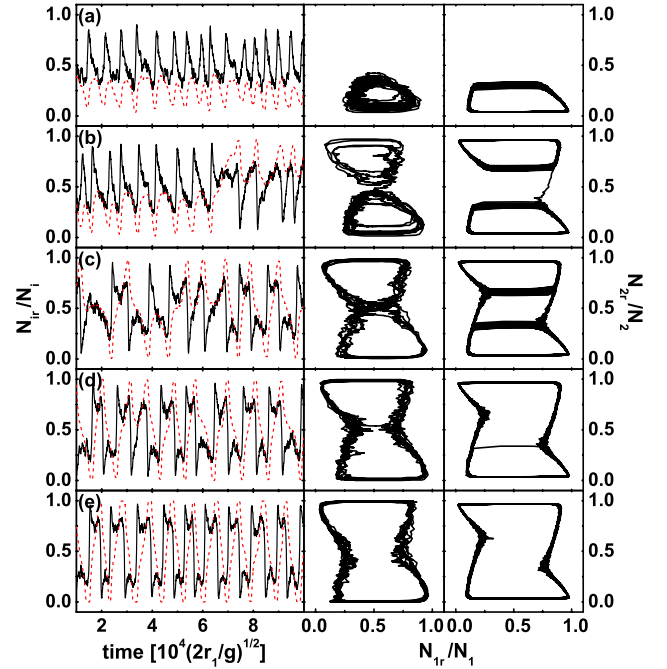
FIG. 5 (color online). Time evolution of populations for the right compartment (left panel: black solid lines for N_{1r}/N_1 and red dashed lines for N_{2r}/N_2 ) and phase trajectories (middle panel) given by MD simulation at \Phi_2 = 0.275 , and v_b = 0.545 (a), 0.535 (b), 0.525 (c), 0.520 (d), and 0.510 (e). The theoretical correspondences obtained from Eq. (2) with noise terms in Eq. (3) are shown in the right panel, with the confining parameters K_1^2 = 3 and K_2^2 = 1 .
