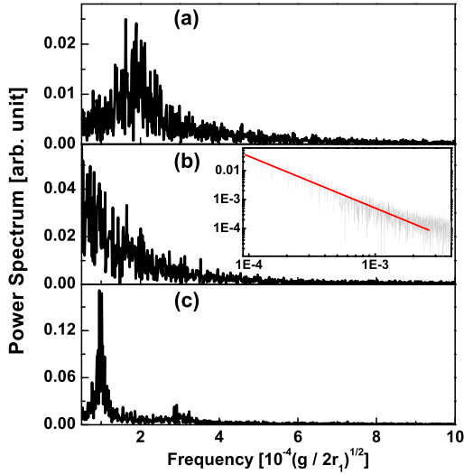
FIG. 6 (color online). Fourier transformation of the time series obtained through simulation in Fig. 5: v_b = 0.545 (a), 0.525 (b), and 0.510 (c). The inset in (b) is a log-scale plot of the data, which shows a 1/f frequency divergence.
