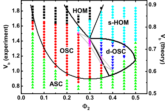
FIG. 1 (color online). Phase diagram in the \Phi_2 - v_b plane: symbols for experimental results and plates separated by solid lines for calculations through FM without noise terms. Irregular oscillations are experimentally observed in the gray polygon.
