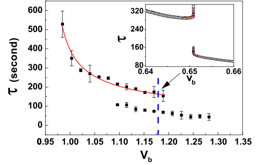
FIG. 4 (color online). Recurrence time for the oscillatory states obtained in experiments. The inset shows the theoretical prediction near the gluing point ( v_b matched according to Fig. 1).
