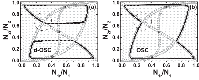
FIG. 3. For \Phi_2 = 0.35 , phase trajectories of the d -OSC state with symmetric double cycles at v_b = 0.651 (a) and OSC state with a single cycle v_b = 0.649 (b) near the gluing point are plotted by solid curves, hollow symbols (circles for dN_{1r}/dt , triangles for dN_{2r}/dt ) show the nullclines of the net flux of both species, and arrows represent the whole flow diagram.
